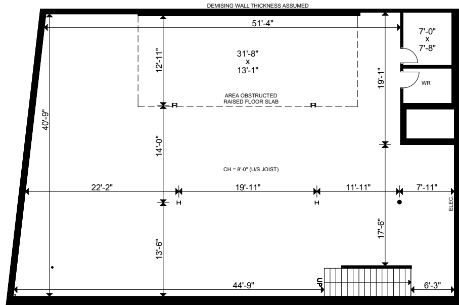
BASEMENT
