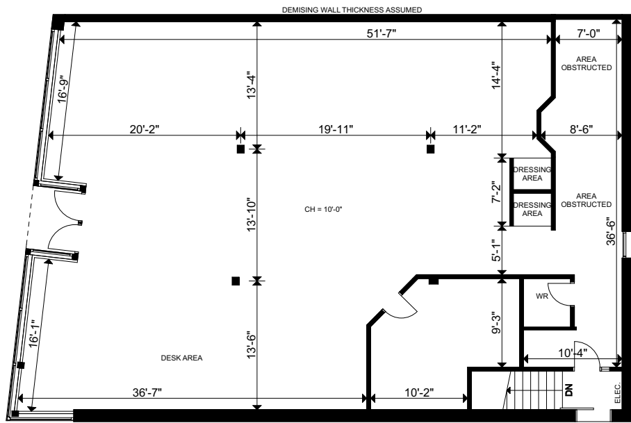
FLOOR 1
