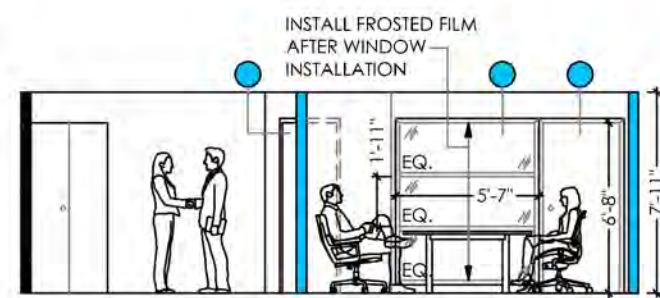
PROPOSED ELEVATION SUITE 800 - LOUNGE & MEETING AREA-1
