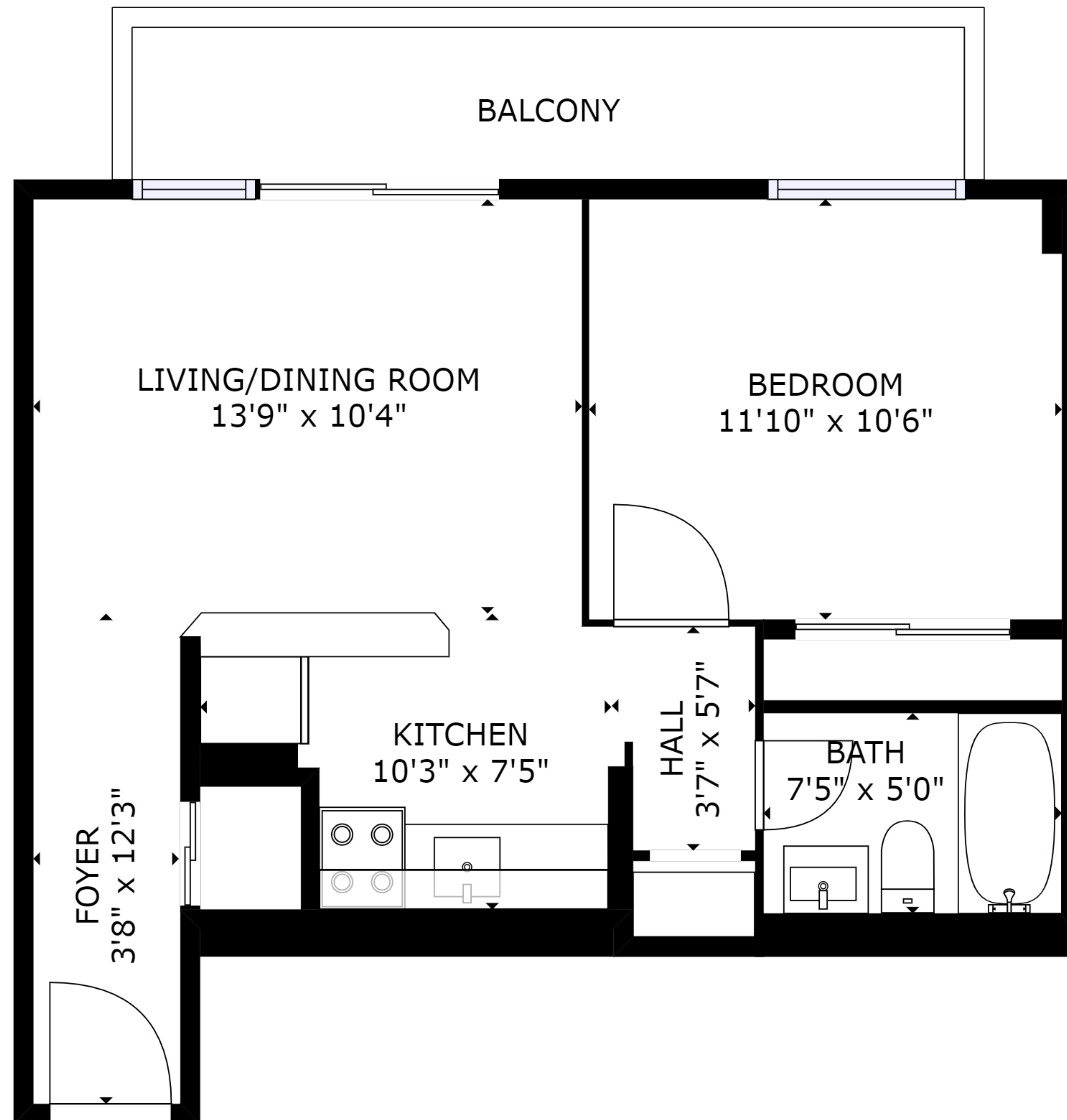
FLOOR 1
