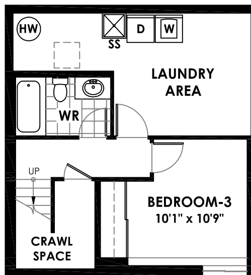
BASEMENT LEVEL
